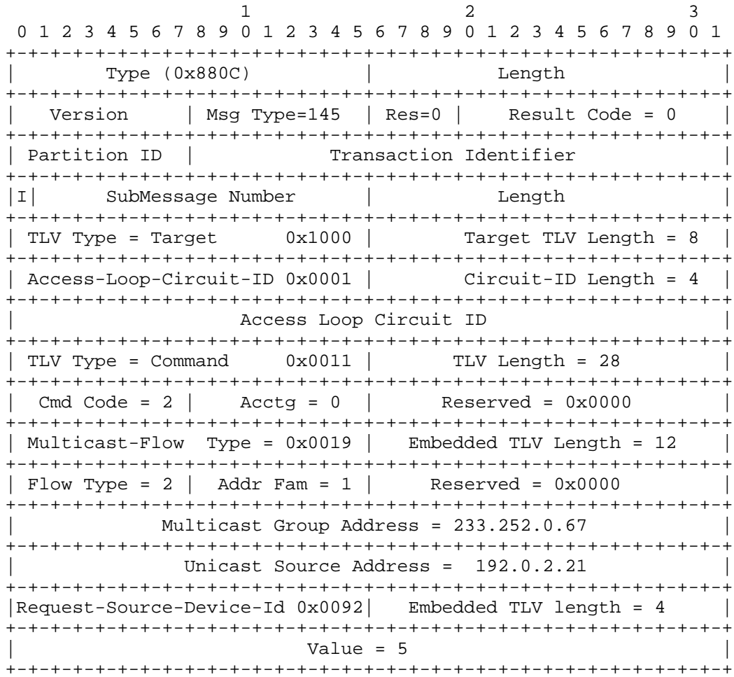
Figure 28: Multicast Admission Control Message Signaling Flow Termination
