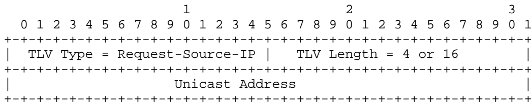
Figure 16: Request-Source-IP TLV
