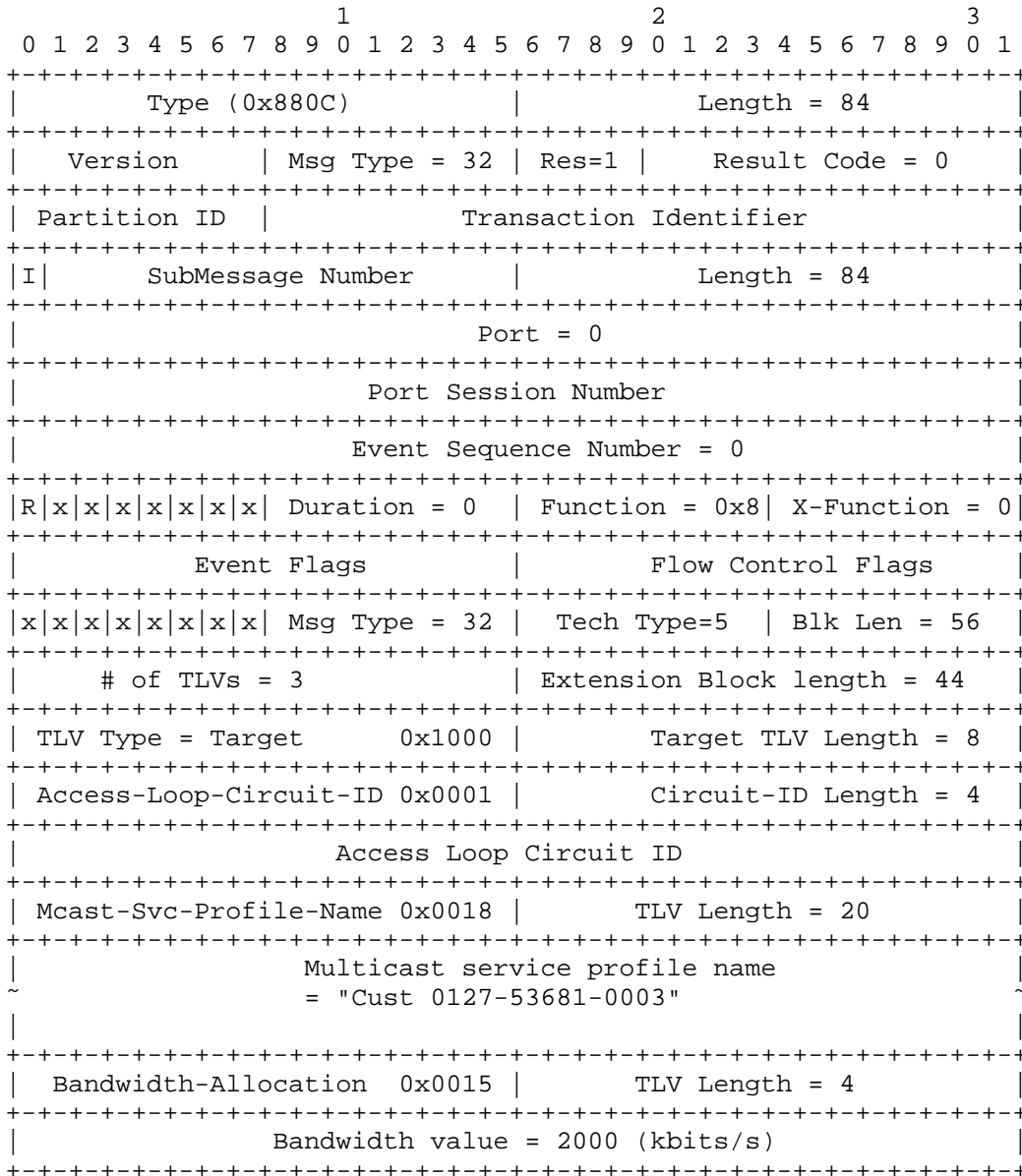
Figure 24: Example Port Management Message
