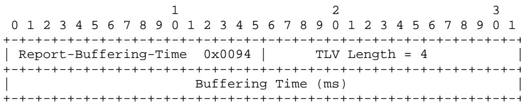
Figure 20: Report-Buffering-Time TLV
