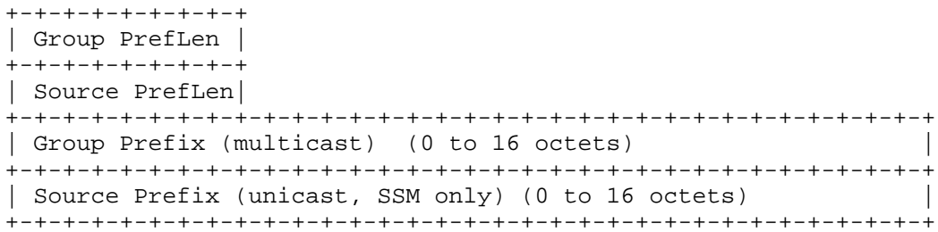
Figure 10: Organization of a Single Multicast Flow Field
