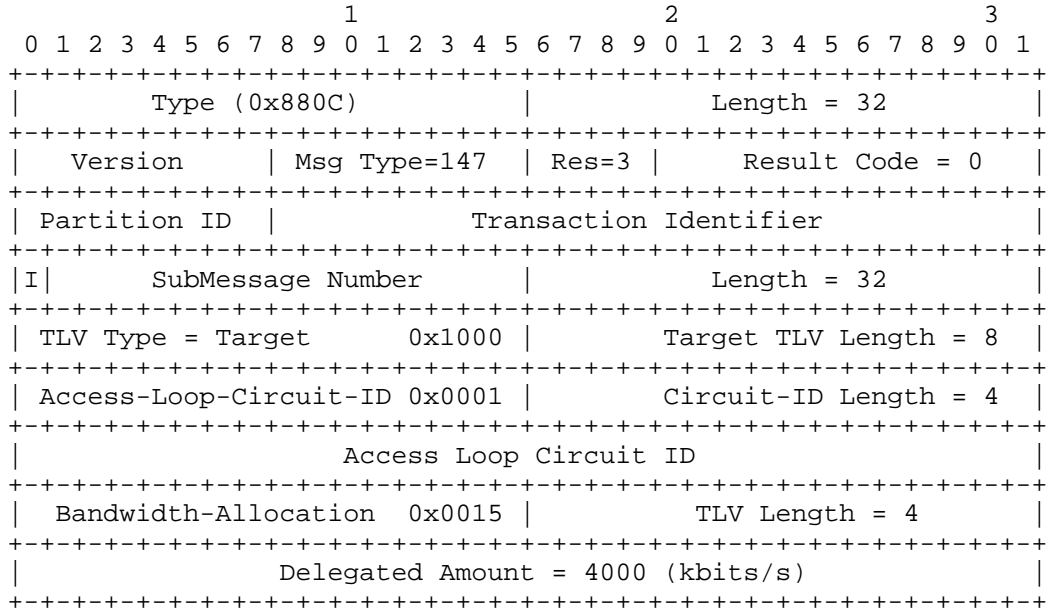
Figure 31: NAS Response, Bandwidth Transfer Message
