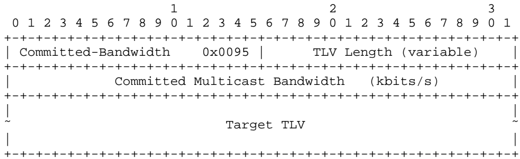
Figure 21: Committed-Bandwidth TLV
