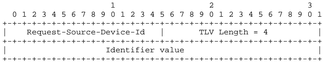
Figure 18: Request-Source-Device-Id TLV
