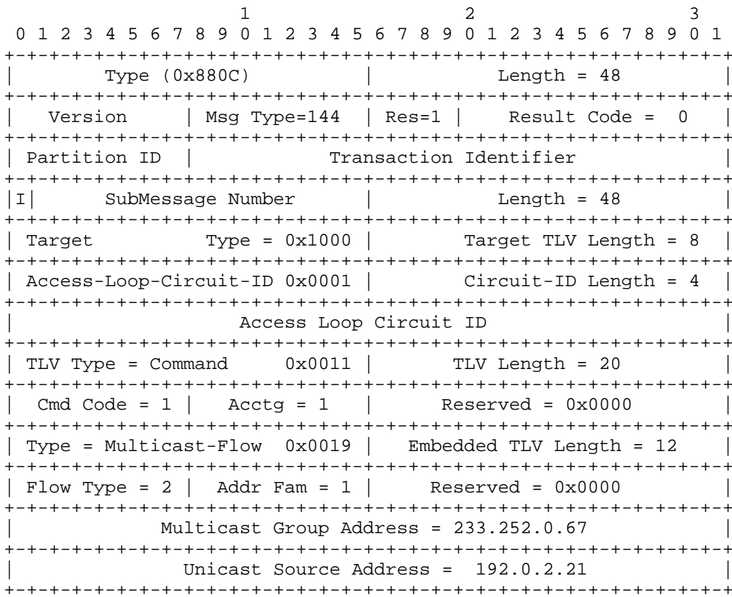
Figure 27: Multicast Replication Control Message Admitting a Flow
