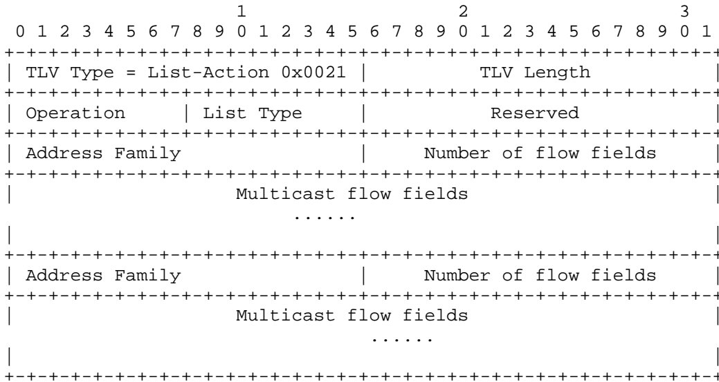
Figure 9: List-Action TLV
