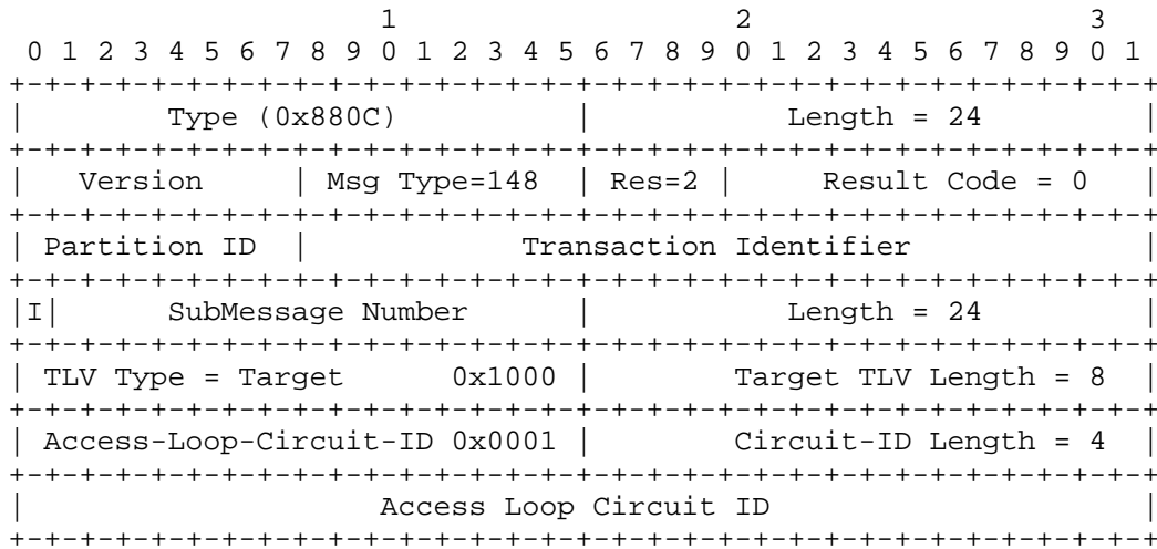
Figure 32: Delegated Bandwidth Query Request Message
