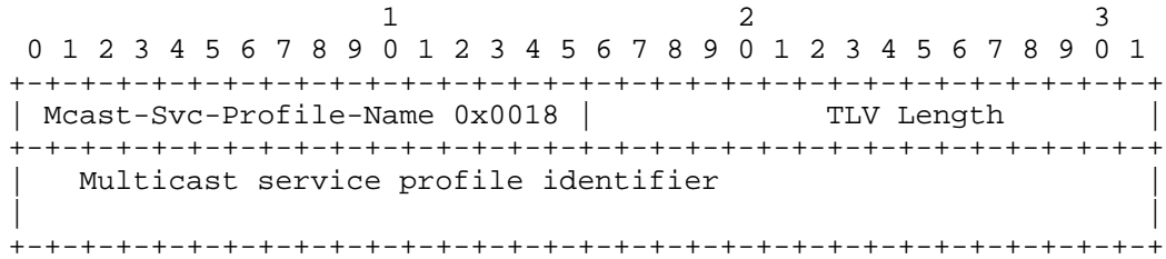
Figure 8: Multicast-Service-Profile-Name TLV
