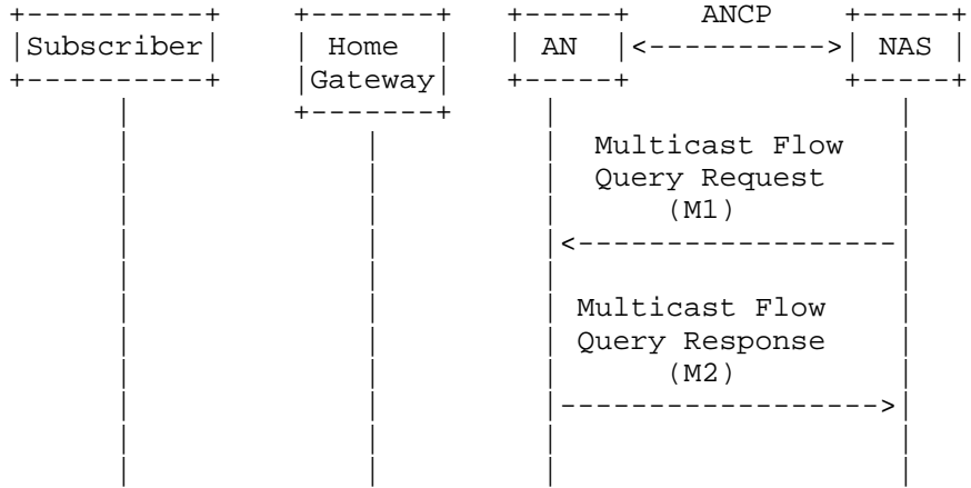
Figure 36: Per-Port Multicast Flow Reporting
