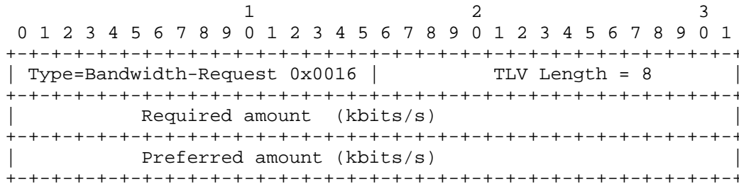
Figure 15: Bandwidth-Request TLV
