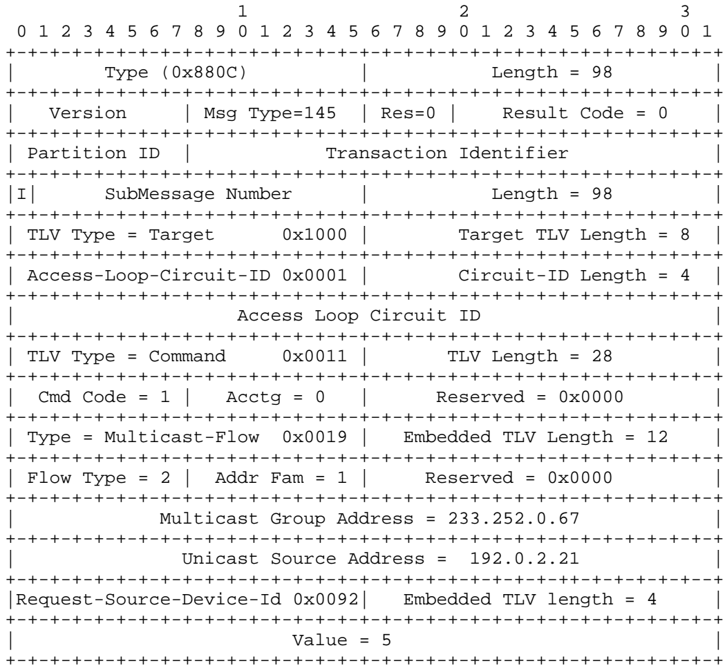
Figure 26: Multicast Admission Control Message Seeking to Add a Flow
