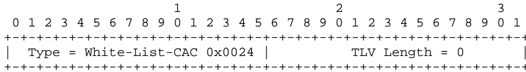
Figure 13: White-List-CAC TLV
