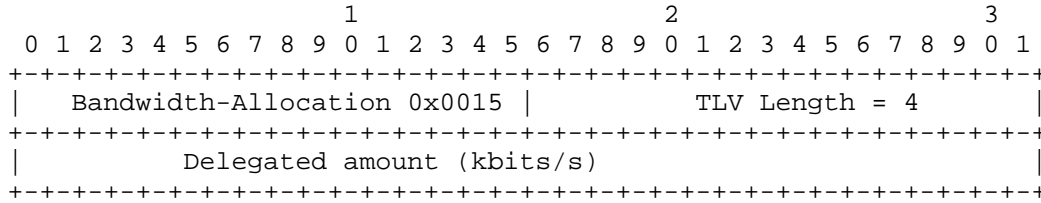
Figure 12: Bandwidth-Allocation TLV
