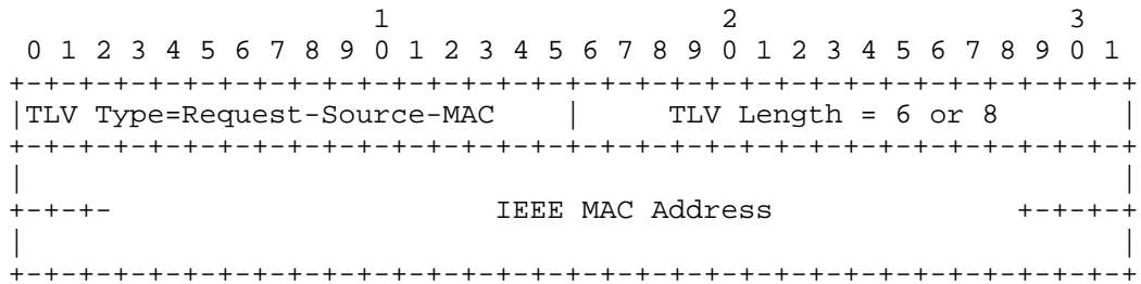
Figure 17: Request-Source-MAC TLV
