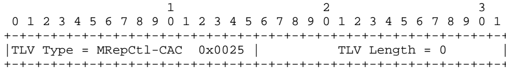
Figure 14: MRepCtl-CAC TLV
