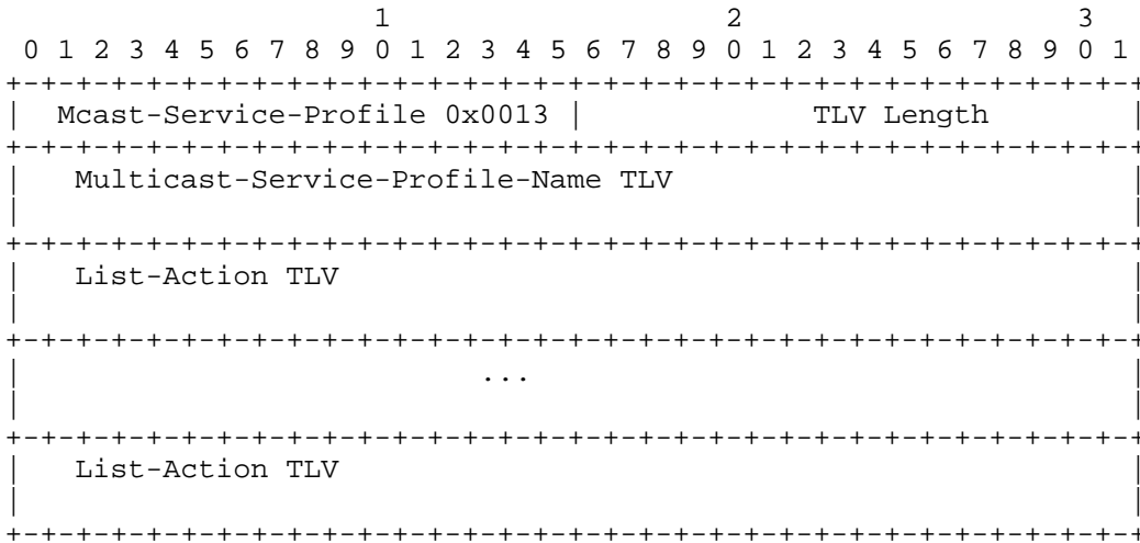
Figure 7: Multicast-Service-Profile TLV
