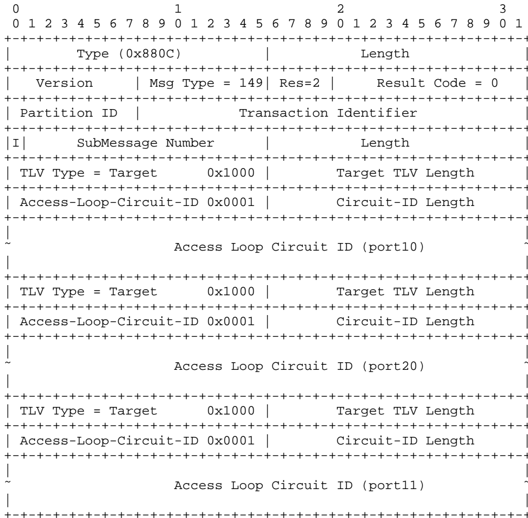
Figure 37: Multicast Flow Query Request Message for Per-Port Multicast Flow Reporting
