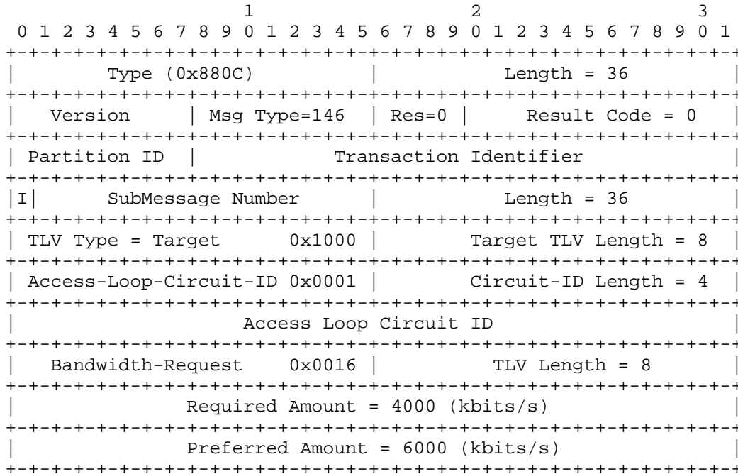
Figure 30: Bandwidth Reallocation Request Message
